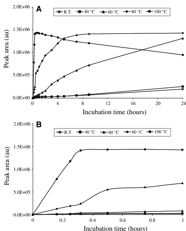
Fig. 2 Reaction trend between FITC and taurine contained in a typical plasma sample performed at different incubation temperatures in a 100 mmol/L sodium phosphate buffer pH 9.5, over 24 h (a). An expanded plot of derivatization curves during the first hour is reported in (b). Results are means of three replicates (CV% < 7%). RT room temperature
