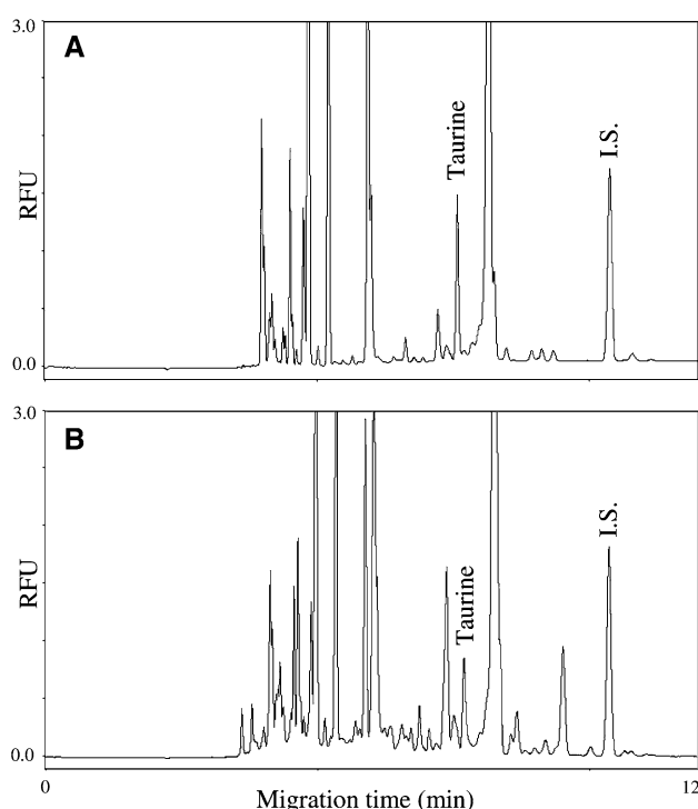
Fig. 6 Electropherogram of taurine contained in energy drink (Red Bull) (a), and Sardinian cow milk (b). The energy drink was diluted 500-fold before analysis
