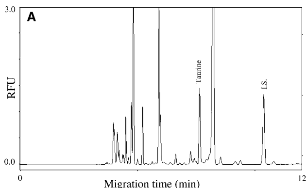
Fig. 1 Typical electropherogram of standard taurine (100 µmol/L) and homocysteic acid (100 µmol/L)
