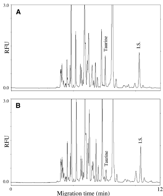
Fig. 4 Representative electropherograms of plasma samples containing elevated (a: 82 \mu\text{mol/L} ) and low (b: 23 \mu\text{mol/L} ) levels of taurine
