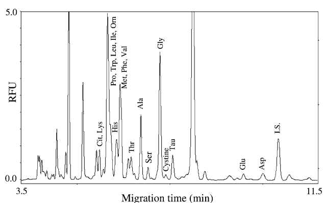
Fig. 5 Electropherogram of a plasma sample showing peak identification of some analytes following amino acid standard co-injection
